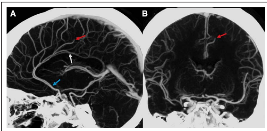
Figure 2. A, Computed tomographic (CT) cerebral angiography thick maximum intensity projection sagittal image showing abrupt cutoff of a callosomarginal artery branch (red arrow) supplying the left supplementary motor area. Also seen are the patent A2 segments of the anterior cerebral arteries (blue arrow) and the patent left pericallosal artery (white arrow) arching around the corpus callosum. B, CT cerebral angiography thick maximum intensity projection coronal image showing abrupt cutoff of a callosomarginal artery branch (red arrow) supplying the left supplementary motor area.
